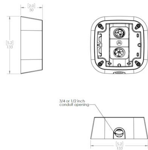
Junction Box
