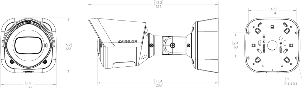
H6A Short Bullet Camera (H6A-BO1-IR)
