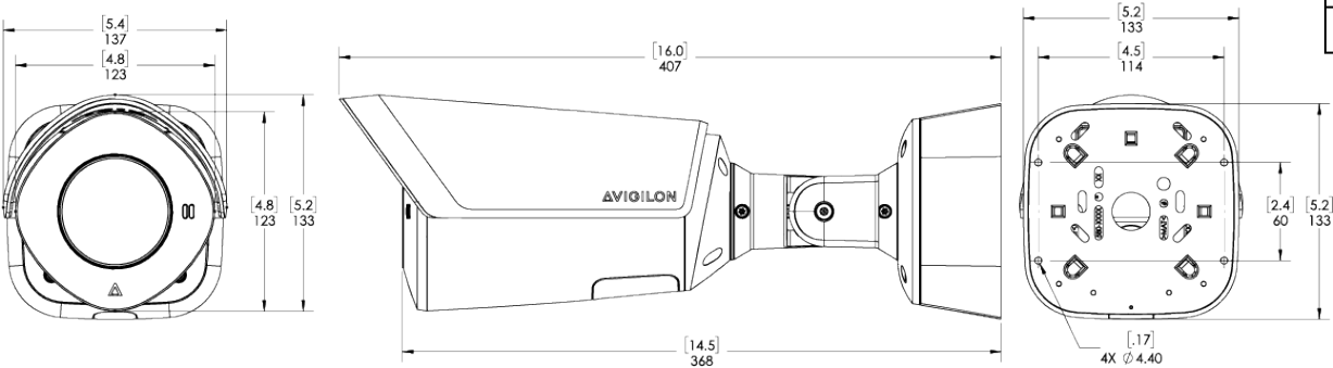
H6A Long Bullet Camera (H6A-BO2-IR)
